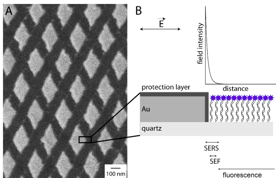
Figure 1: Schematic illustration of gold nanorhombic plasmonic substrate. (A) The SEM image shows the periodically patterned gold surface. (B) Due to the interaction of the incident light with a metallic nanoparticle, surface plasmons are generated on the metal dielectric interface yielding a strong electromagnetic field with an evanescent decay on the nanoparticle surface. The strong electromagnetic field enhancement is employed for the effective enhancement of the Raman cross section (SERS) and the fluorescence (SEF), as indicating by the arrows.
