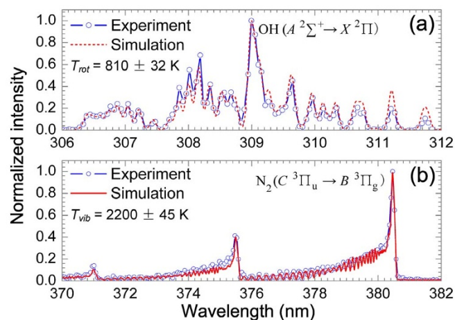
Figure 5 | The comparison of experimental and simulated spectra of (a) \text{OH}(A^2\Sigma^+ \rightarrow X^2\Pi, \Delta v = 0) transition for T_{\text{rot}} measurement and (b) \text{N}_2(C^3\Pi_u \rightarrow B^3\Pi_g, \Delta v = -2) transition for T_{\text{vib}} measurement.
