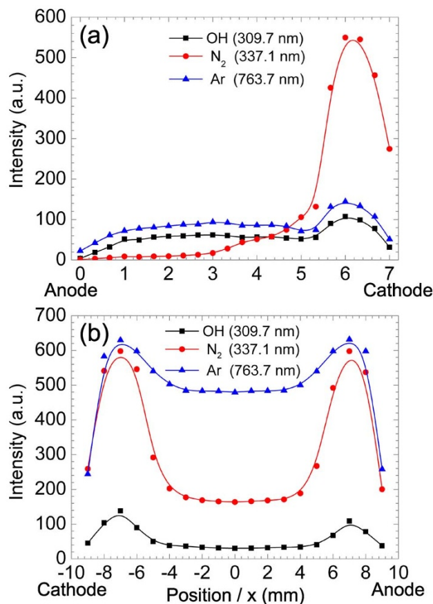
Figure 6 | Emission profiles of the radical OH (309.7 nm), excited \text{N}_2 (337.1 nm), and excited argon (763.7 nm) along x axis with a longitudinal (a) and transverse (b) electric field applied on the flowing gas, respectively.
