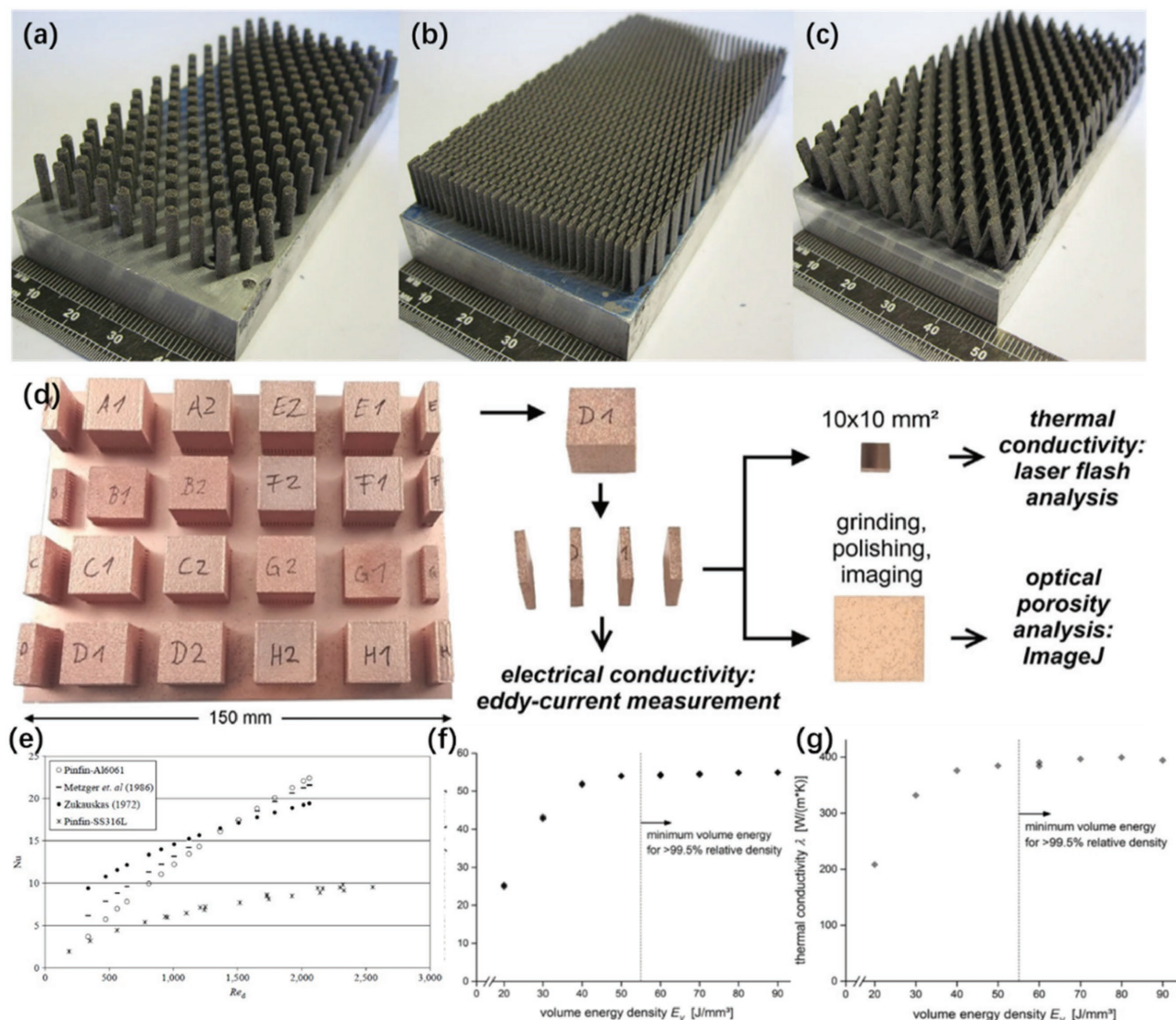
Figure 26. AM fabricated heat sinks (a) Pinfin-Al6061; (b) Diamond-Al6061; (c) V-Al6061. Reproduced with permission. [275] Copyright 2007, Emerald Group Publishing Ltd. (d) Procedures for SEBM fabricated copper sample preparation. Reproduced with permission. [277] (e) Heat transfer performance of Pinfin, Diamond and V geometries investigated. Reproduced with permission. [275] Copyright 2007, Emerald Group Publishing Ltd. (f) Electrical and (g) thermal conductivities of SEBM fabricated copper samples with respect to volume energy density (various relative densities). Reproduced with permission. [277]
