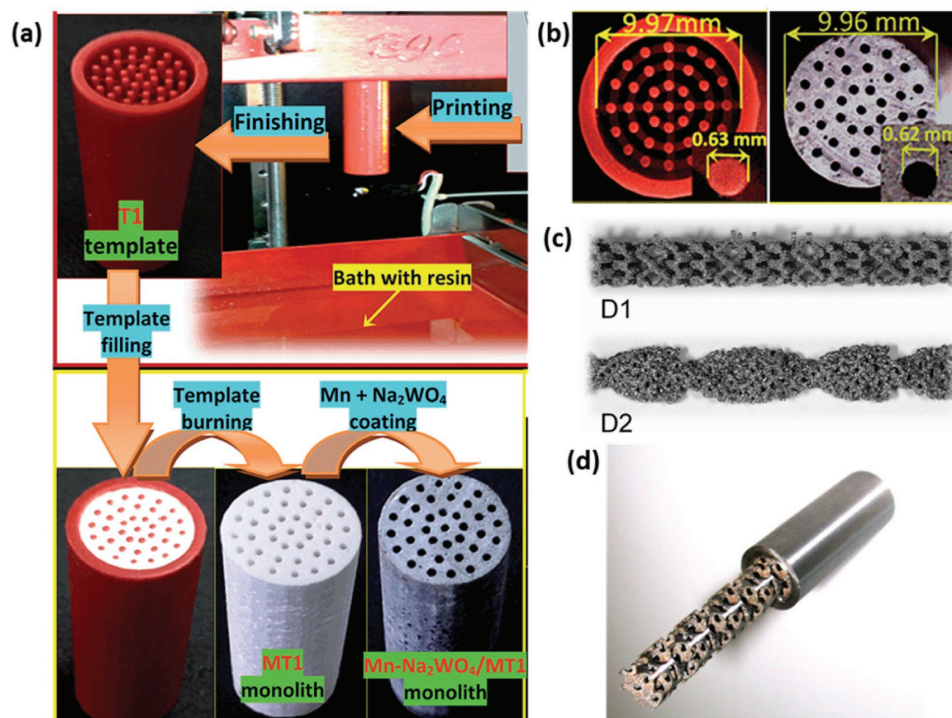
Figure 16. Schematics showing monolithic catalyst preparation. a) SLA printing of a polymer template (T1), followed by filling the template with α-Al 2 O 3 paste, burning of polymer template and coating the resulting monolith (MT1) with Mn-Na 2 WO 4 , b) optical images of dimensions of SLA fabricated template and monolithic catalyst. Reproduced with permission. [186] Copyright 2016, Royal Society of Chemistry. c) Catalytic static mixers (CSMs) fabricated via EBM. Reproduced with permission. [188] Copyright 2016, Royal Society of Chemistry. d) Uncoated designed porous structure reactor (DPSR) fabricated via SLS. Reproduced with permission. [189] Copyright 2015, Elsevier.
