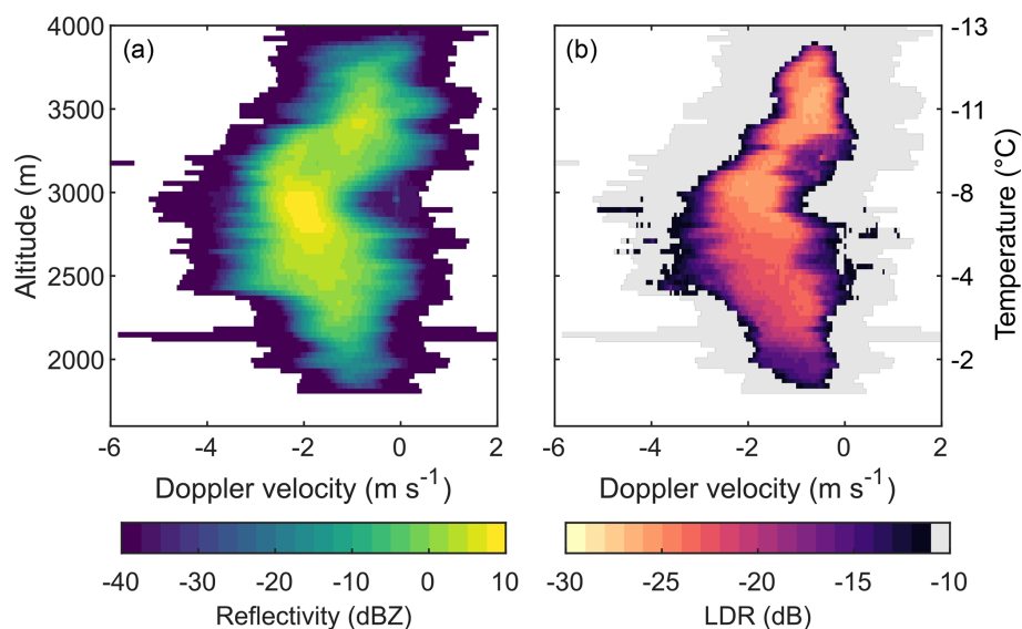
Figure 10. Vertical profile of the radar reflectivity (a) and LDR (b) Doppler spectra along the LDR fallstreak at 18:00 UTC averaged over 1 min (see red line in Fig. 3d). LDR values larger than -10 \text{ dB} are shown in gray. The temperature profile measured by the radiosonde is shown on the right y axis.
