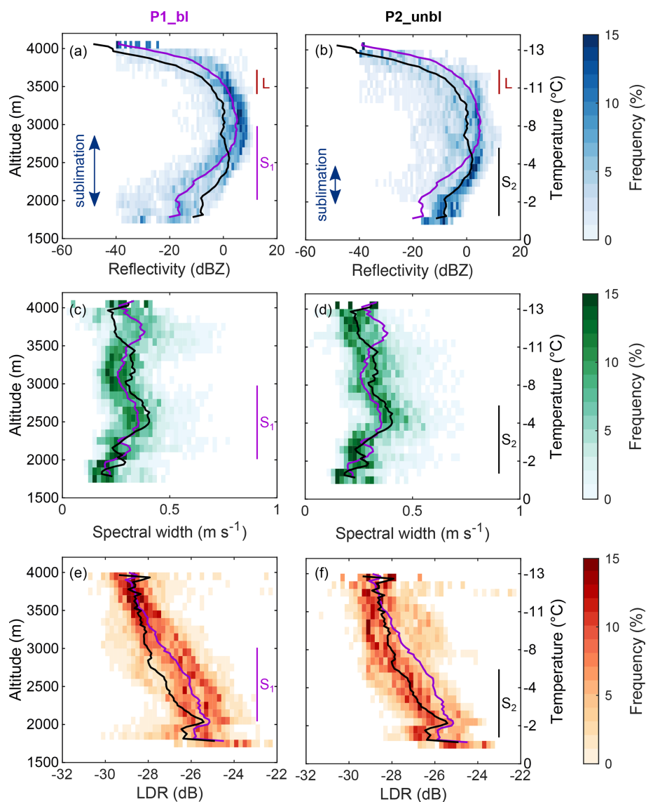
Figure 8. CFADs of the radar reflectivity (a, b), spectral width (c, d) and linear depolarization ratio (e, f) averaged over sub-periods of P1_bl (left; 17:00–17:45 UTC) and P2_unbl (right; 17:45–18:30 UTC). The following bin sizes were applied: (1) radar reflectivity from -40 to 20 dBZ in 1 dBZ intervals, (2) spectral width from 0 to 0.8 \text{ m s}^{-1} in 0.02 \text{ m s}^{-1} intervals and (3) LDR from -32 to -22 dB in 0.2 dB intervals. A height interval of 100 \text{ m} was used for all radar properties. The solid lines represent the mean vertical profile of P1_bl (purple) and P2_unbl (black). The temperature profile measured by the radiosonde is shown on the right y axis. The extent of the shear layer ( S_1 , S_2 ; from wind profiler), the supercooled liquid layer (L; from cloud lidar) and the sublimation layer (blue arrow; from cloud radar) is indicated.
