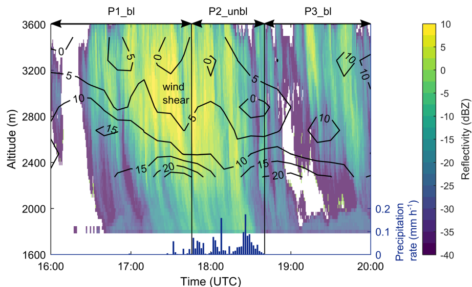
Figure 9. Temporal and spatial evolution of the vertical wind shear (in \text{m s}^{-1} \text{km}^{-1} ; black contour lines), the radar reflectivity (colored area) and the precipitation rate (blue bars). The wind shear was calculated from the wind profiler observations (Fig. 5), and the precipitation rate was measured with a disdrometer at Wolfgang (1630 m).
