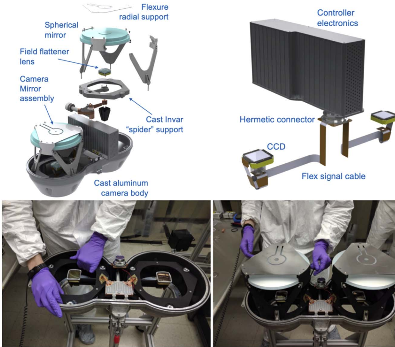
Figure 10. The upper renderings show the anatomy of the VIRUS camera assembly. The top left panel displays how the Invar-36 camera-mirror assembly integrates with the “spider” support for the detector and field flattener lens in the cryostat housing. All parts of the camera-mirror assembly are Invar-36. The mirrors have a spherical back for lightweighting. The Invar blade flexures at the top provide radial support and are bonded to flats at the centers of the mirror backs, with mirror adjustments at the three corners that are accessed via vacuum feed-throughs on a temporary adjuster back, during alignment. The top right panel shows the electronics signal path via the double-sided flex circuit connecting each detector to the common four-channel readout electronics (controller). The controller box mounts to a hermetic vacuum feed-through connector that mounts in the cryostat cover (not shown). The bottom two panels show two stages of the assembly of a VIRUS camera. The left panel shows two CCDs with integrated field flattener lenses mounted on cast Invar “spiders” with cold links and flex circuit, integrated in the cast aluminum camera body. The right panel displays the two camera-mirror assemblies integrated, prior to installation of the camera cover, which is also cast from aluminum. Figure partly adapted from Hill et al. (2018b), Figure 4.
