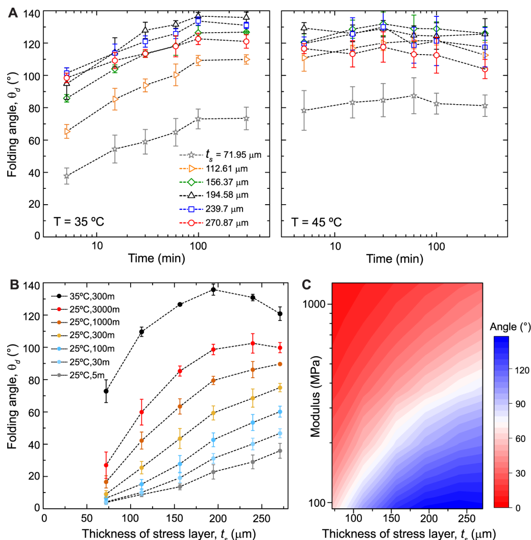
Figure 4. Bilayer characteristics at elevated temperatures and design guidelines. (A) Plots show the time dependence of the folding angle of the bilayer system used for creating folds at 35 and 45 °C. The folding angle shows little variation past 100 min at 35 °C. Samples approach a steady-state folding angle after \sim 5 min at 45 °C. (B) The folding angle is shown as a function of the stress layer thickness at various time instants at 25 °C. The black curve shows the saturated folding angle at 35 °C (after 300 min). Note that the optimum thickness of the stress layer for creating larger folds changes with time (due to a larger creep compliance). (C) Finite-element analysis (FEA) predictions of the folding angle based on the geometry and time (or equivalently elastic modulus, from Figure 3B). Comparison with the experimental values and Timoshenko's bilayer model is explained in the Supporting Information and in Figure S5.
