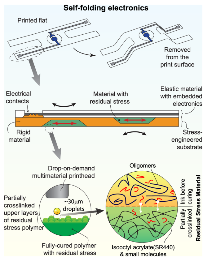
Figure 1. Schematic representation of spontaneously folding electronics achieved by multimaterial 3D-printing. The composites containing active electronics, metallic traces, and the substrate are fully 3D-printed. On removing the 3D-printed structure from the print platform, the composite spontaneously folds in a shape based on the locally engineered residual stress, requiring no stimulus at room temperature. At the heart of this scheme is a UV-curable ink containing high-elongation acrylate oligomers and short-chain monomers (such as isooctyl acrylate). As a part of the layer-by-layer inkjet-based 3D-printing process, each previously cured (lightly cross-linked) layer, \sim 17 \mu\text{m} thick, is exposed to uncured ink from the subsequent layers. The small molecules from the ink swell the underlying cured layers and create a local residual stress. Both the circular close-ups shown in the bottom only show the residual stress material before and after curing; the rigid material is not linked to the stress-generation mechanism. The role of each ink component is shown in Figure S1. This material, which is used to directly write residual stress in a volume, is combined with rigid UV-curable acrylates to create both concave and convex folds of the desired angles by controlling the material placement and geometry in the design. The active electronics are linked by a stretchable conductor all printed within the same system.
