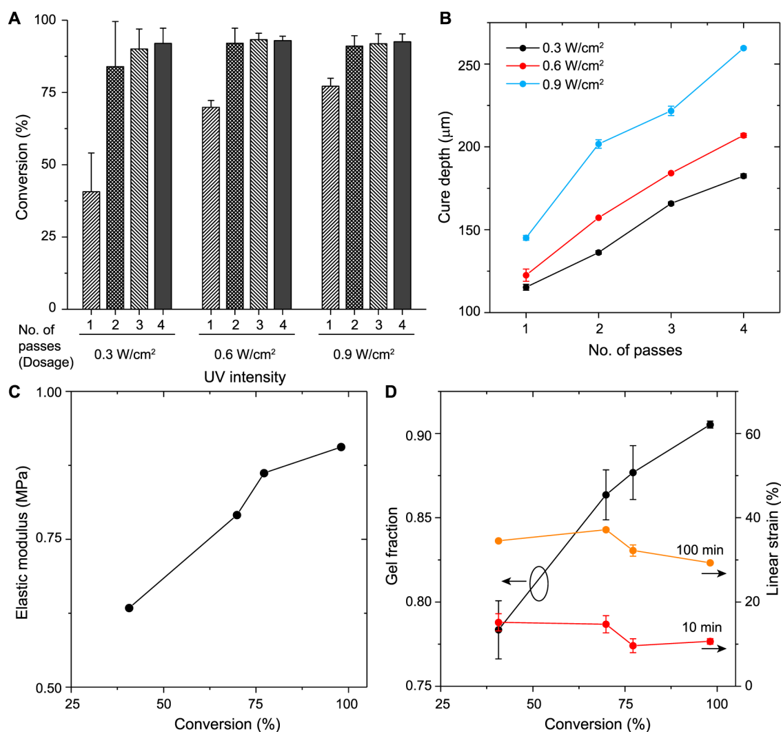
Figure 2. Residual stress polymer and process characterization. (A) The double-bond conversion percentage is calculated as a function of the UV light intensity and the number of curing passes from the Fourier transform infrared (FTIR) attenuated total reflection (ATR) measurements on the surface of the samples (three samples for each data point). The absorbance values corresponding to the reactive double bond “ -\text{CH}=\text{CH}_2 ” group are normalized with respect to the “ -\text{COO}- ” group to obtain the reaction conversion (40). The sample FTIR spectra are shown in Figure S2. (B) Plot of the cure depth measured as a function UV light intensity and the number of passes. (C) Elastic modulus values are measured for the samples after one UV curing pass at various light intensities (0.3, 0.6, and 0.9 \text{W cm}^{-2} using the printer and \sim 14 \text{ W cm}^{-2} using a high-intensity broadband source, UV fusion). (D) Measured linear expansion in one dimension as a function of double-bond conversion for different swelling times (samples are \sim 125 \mu\text{m} thick). The samples are prepared using single curing passes with varying UV light-emitting diode (LED) intensities. As printed, the samples shrink by <1\% typically. These samples with one-shot curing are expected to show isotropic swelling. The plot also shows the measured gel fraction of these samples.
