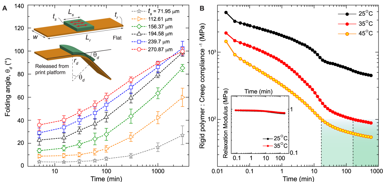
Figure 3. Temporal characteristics of the bilayer system used for creating folds. (A) Inset shows a bilayer stack where the material with the residual stress (green, called residual stress material in text) causes the underlying substrate made of the rigid material to bend. The plot shows the time evolution of \theta_d , the bending angle at standard room temperature (25 °C) once the sample is removed from the print platform. The different curves show the bending angle as a function of time for varying thickness of the material with residual stress, t_s . For these tests, the thickness of the rigid polymer is t_r = 99.9 \pm 4.3 \mu\text{m} , width W = 3.25 \text{ mm} , and length L_r = 15 \text{ mm} and L_s = 4 \text{ mm} . The folding angle does not settle even after 3000 min. (B) The plot shows the inverse of the creep compliance of the rigid material at 25, 35, and 45 °C. The material shows a rapid increase in the compliance until \sim 30 \text{ min} , after which the increase in creep compliance settles to a slower rate. The modulus drops by more than 1 order of magnitude between the start and 10 h into the creep test. With the rigid material having a glass transition temperature ( T_g ) close to the room temperature, the inherent stiffness of the material drops drastically as the temperature increases above 25 °C. The shaded region shows the time it takes for the inverse creep compliance to drop below 100 MPa. The inset shows the relaxation modulus of the stress layer material. The relaxation modulus shows a negligible drop after 200 min (of the stress-relaxation experiment). Further, there is no significant change in the base stiffness of the material as the temperature is increased to 35 °C because the material is well into the rubbery regime. The glass transition measurements for the two materials are included in Figure S3.
