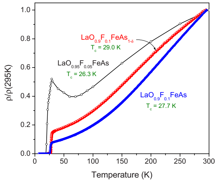
Figure 3. T dependence of the normalized resistivity for the As deficient (red circles), the reference sample (blue circles), and an underdoped sample ( \circ ) taken from [37].
