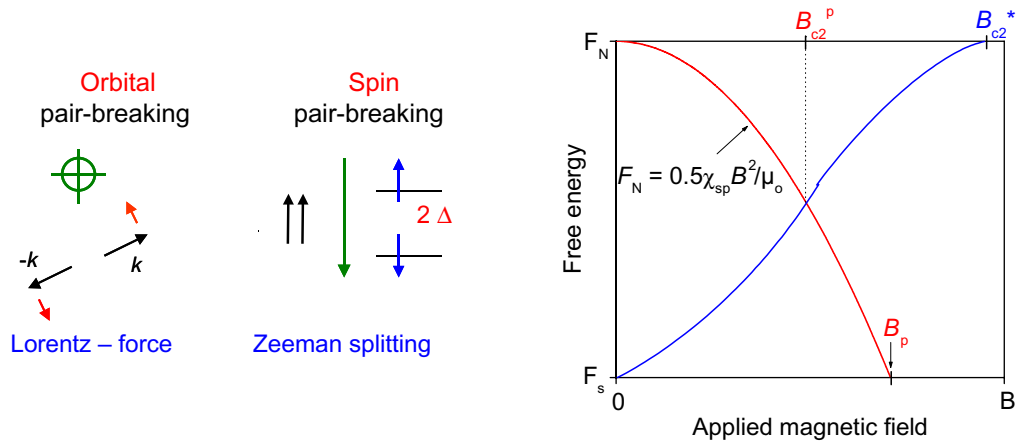
Figure 10. Schematic view of the magnetic field affecting a Cooper-pair (left). Pair breaking due to the Lorentz force acting via the charge on the momenta of the paired electrons ( orbital pair-breaking) or due to the Zeeman effect aligning the spins of the two electrons with the applied field ( spin pair-breaking). Field dependence of the Gibbs-free energy schematically (right). The free energy in the normal state with Pauli spin susceptibility \chi_{sp} (parabolic red line) crossing the zero-field free energy in the superconducting state at the Pauli limiting field B_p and without \chi_{sp} (upper horizontal line). Blue curve: free energy of a type-II superconductor crossing the normal state at B_{c2}^* or B_{c2}^P .
