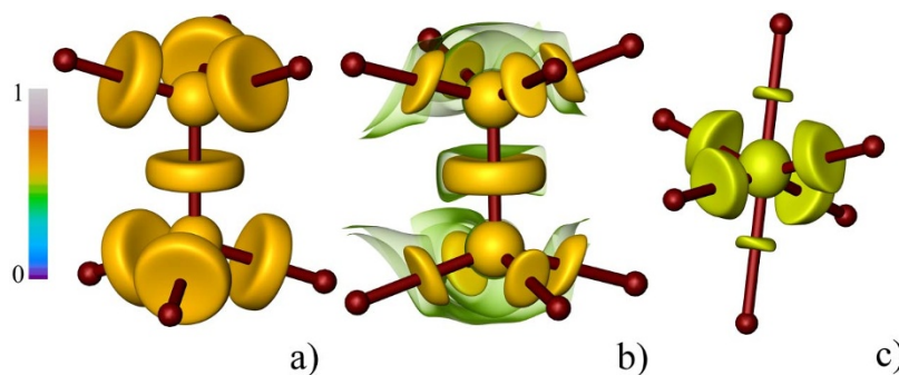
Figure 4 | Evolution of the bonding situation from diamond to \beta -tin type over bct-5. The ELF map is showing four bond attractors for diamond Ge (a, \eta = 0.58 ), one + four bond attractors for bct-5 (b, \eta = 0.53 , transparent green isosurface \eta = 0.48 ), two + four bond attractors for \beta -tin (c, \eta = 0.51 ).
