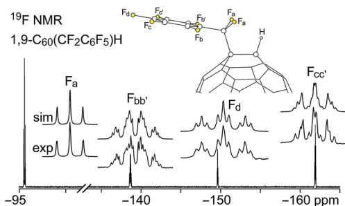
Fig. 3 Experimental and simulated 376.5 MHz ^{19}\text{F} NMR spectra of HPLC-purified 1,9- \text{C}_{60}(\text{CF}_2\text{C}_6\text{F}_5)\text{H} (1) in \text{CDCl}_3 . Chemical shifts and coupling constants are listed in Table S-2.†
