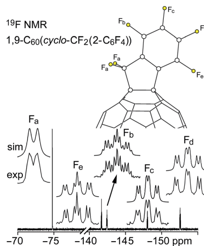
Fig. 4 Experimental and simulated 376.5 MHz ^{19}\text{F} NMR spectra of HPLC-purified 1,9- \text{C}_{60}(\text{cyclo}-\text{CF}_2(2-\text{C}_6\text{F}_4)) (2) in \text{CDCl}_3 . Chemical shifts and coupling constants are listed in Table S-2.†
