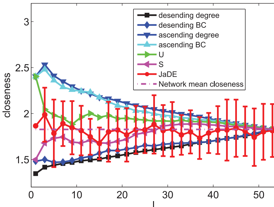
Figure 9. The mean values of closeness information of driver nodes with various l under different schemes when minimizing \sigma . doi:10.1371/journal.pone.0041375.g009
