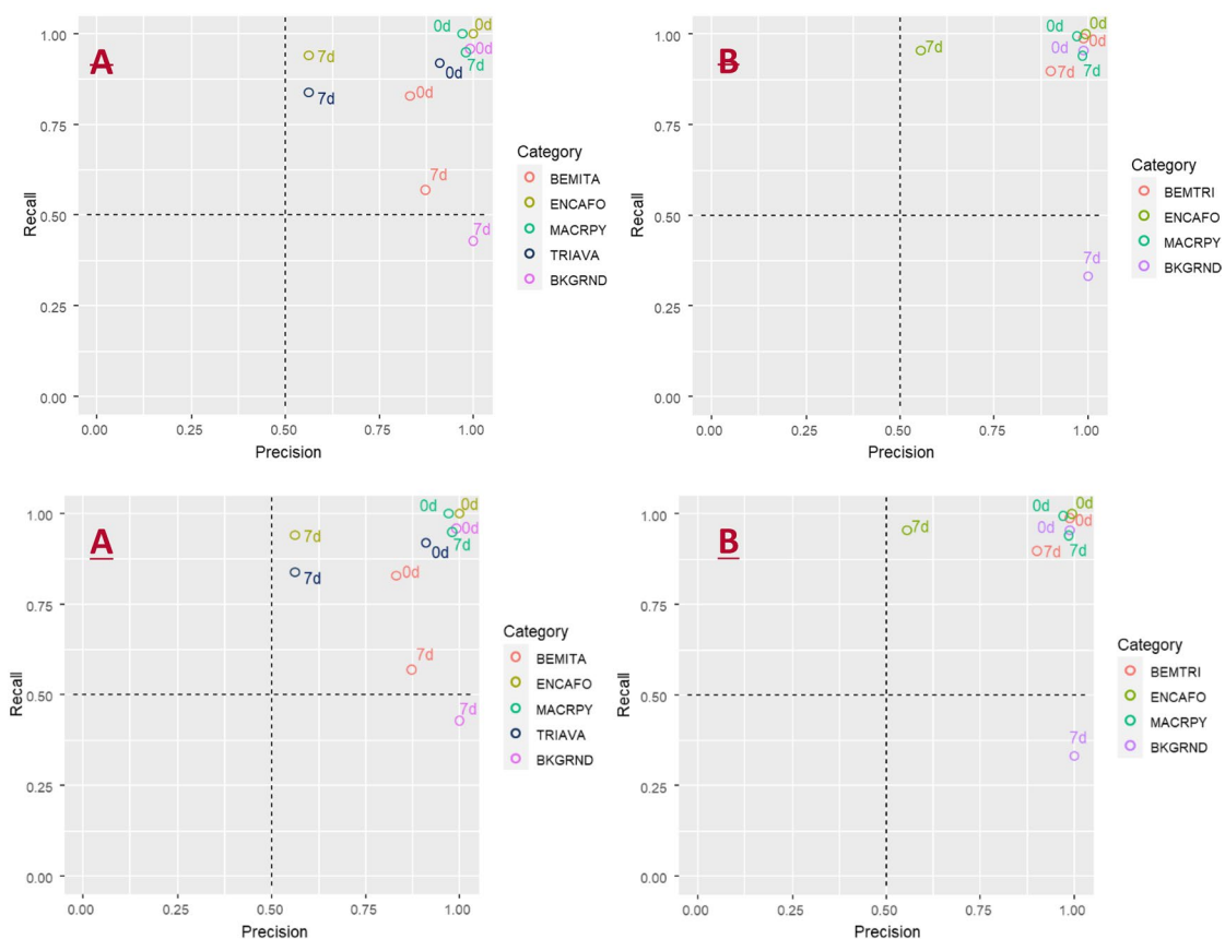
Figure 1. Recall-precision plots for (A) model 164 with no categorical pooling and (B) with categorical pooling. 7d = Lab7d dataset, 0d = Lab0d dataset, BEM-TRI = pooled class of B. tabaci and T. vaporariorum . The graphs were generated using ggplot in R 20,21 .
