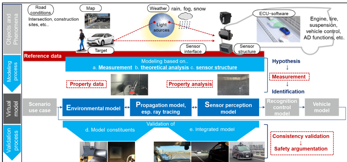
Abbildung: Einbettung der Sensormodelle in den VIVID Modellierungs- und Validierungsprozess. (Quelle: The role of sensor and environmental modeling in the virtual validation tool chain for controlling risks of automated and connected driving , VIVID Presentation, Mobility Innovation Week/Tokyo, Tsukuba, Nov 14-17, 2023)
