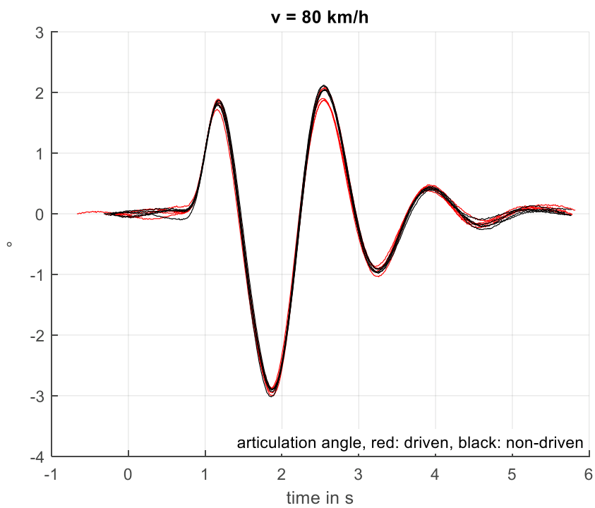
Figure 24: Manufacturer B, 80 km/h
