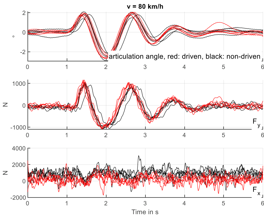
Figure 15: Manufacturer A, 80 km/h
