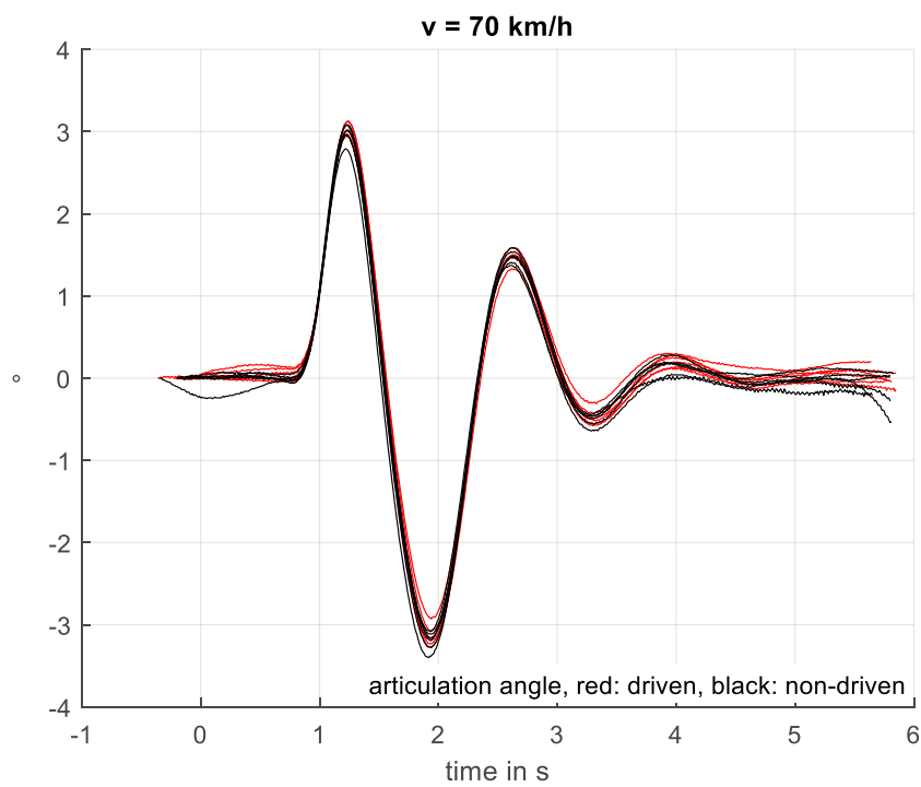
Figure 22: Manufacturer B, 70 km/h
