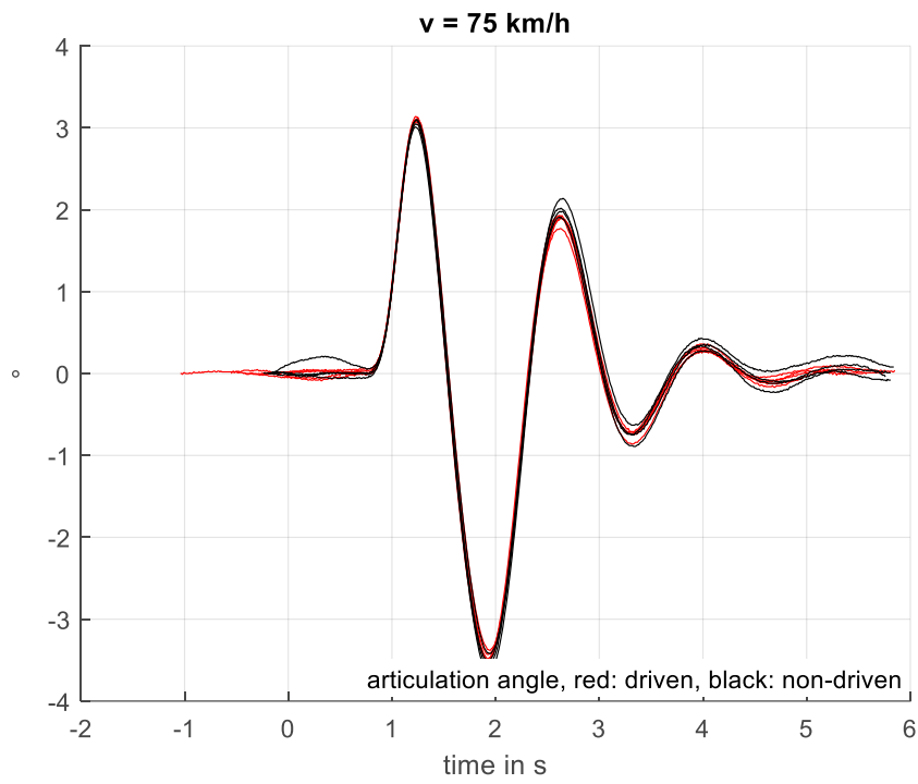
Figure 23: Manufacturer B, 75 km/h
