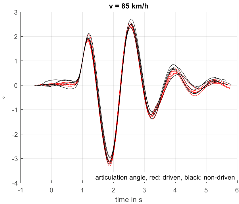
Figure 25: Manufacturer B, 85 km/h
