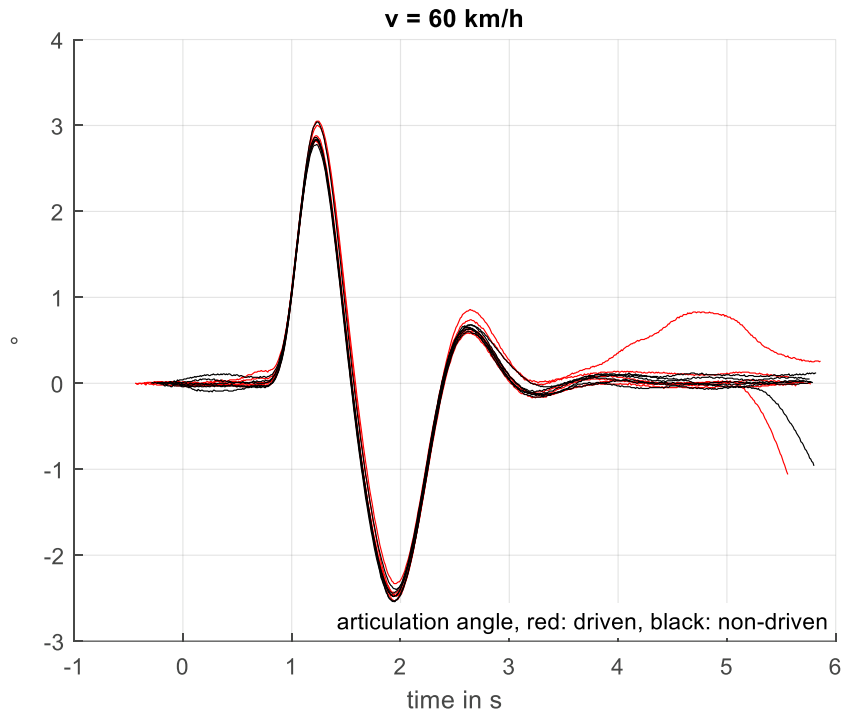
Figure 20: Manufacturer B, 60 km/h
