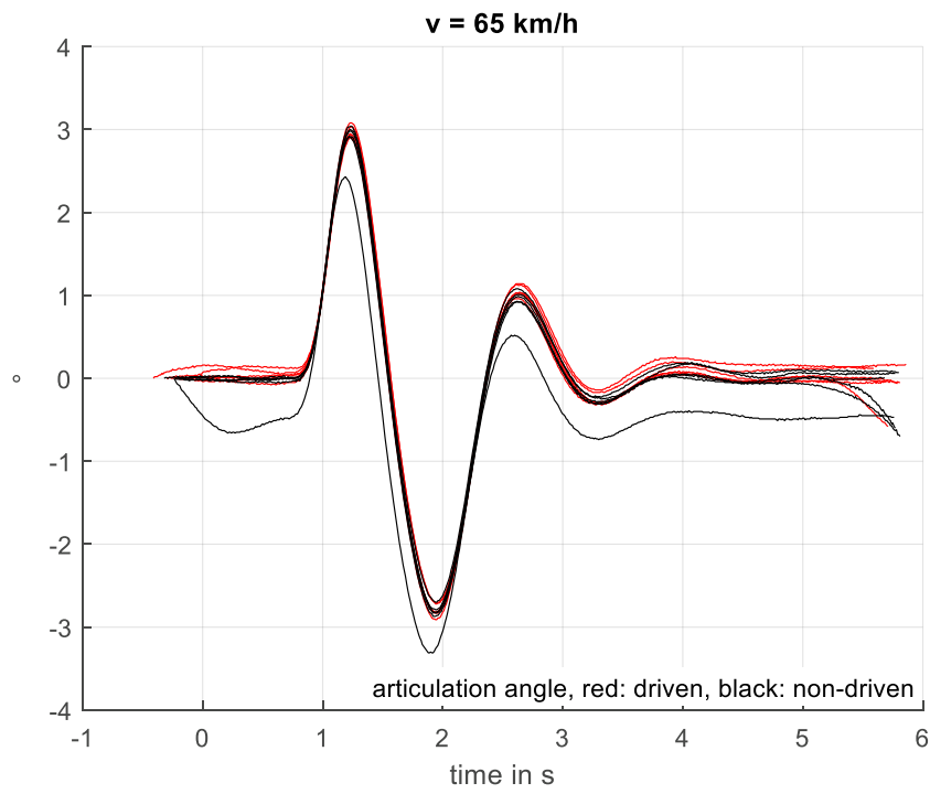
Figure 21: Manufacturer B, 65 km/h
