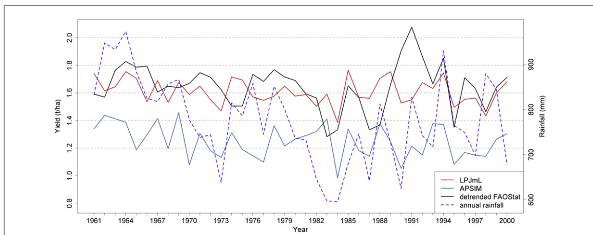
Figure 7. Sample time-series (1961–2000) of detrended national mean maize yields from FAO ( t\ ha^{-1} ), annual rainfall from CRU climate (mm) and simulated mean area-weighted national maize yields ( t\ ha^{-1} ) from model LPJmL CRU-FAO-Variable and APSIM CRU-FAO-Variable. See supplementary material S2 for details on calculating and removing the trend.
