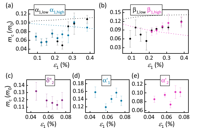
FIG. 7. Strain evolution of the cyclotron masses extracted from the T dependence of the Fourier peaks for different orbits. Dotted lines represent the calculated values.
