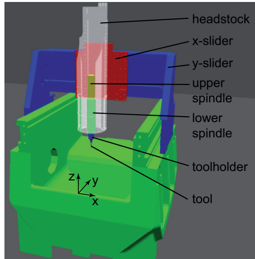
Figure 7: Multi-body system representing the milling machine.
