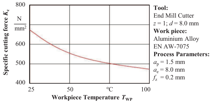
Figure 5: The dependency of the specific cutting force K_c on the preheating of the work piece.
