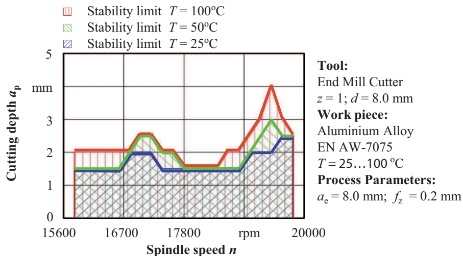
Figure 6: Stability limits in dependency of the temperature.
