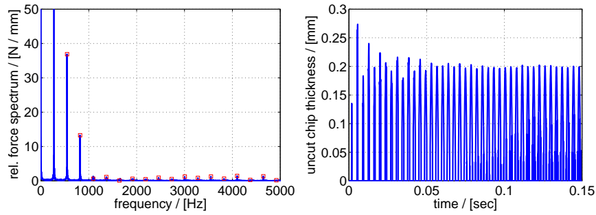
Figure 11: Relative cutting force spectrum and evolution of the uncut chip thickness corresponding to a stable cut.
