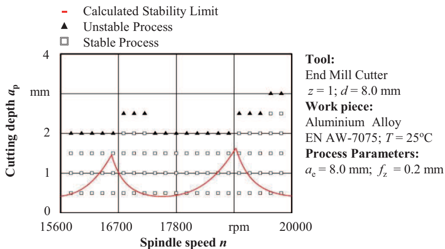
Figure 3: Stability plot for a feed-rate-per-tooth of f_z = 0.2 mm.
