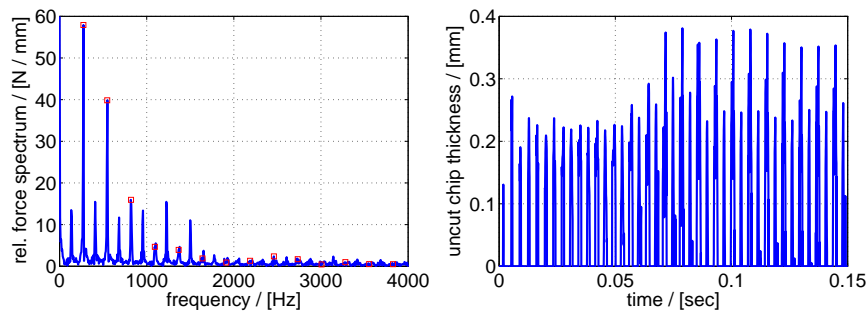
Figure 13: Relative cutting force spectrum and evolution of the uncut chip thickness corresponding to an unstable cut due to a supple work piece.
