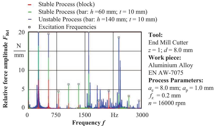
Figure 4: Comparison of stability behavior considering different geometries.
