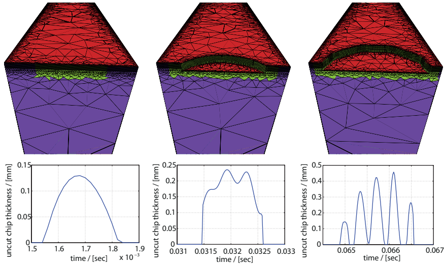
Figure 10: Example for the material removal simulation, i.e. the evolution of the work piece shape, and the corresponding uncut chip thickness in case of an unstable cut.
