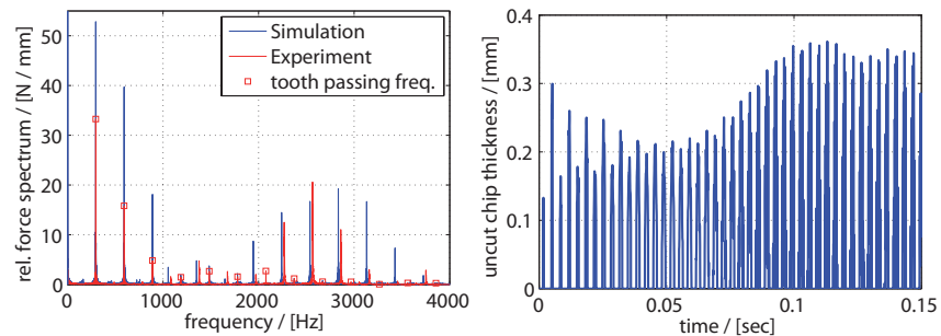
Figure 12: Simulated and measured relative cutting force spectrum and evolution of the uncut chip thickness corresponding to an unstable cut.
