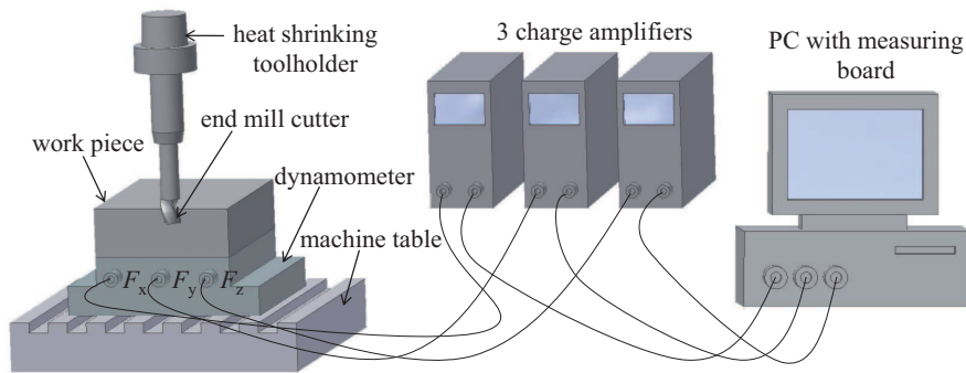
Figure 1: Experimental setup for machining tests.
