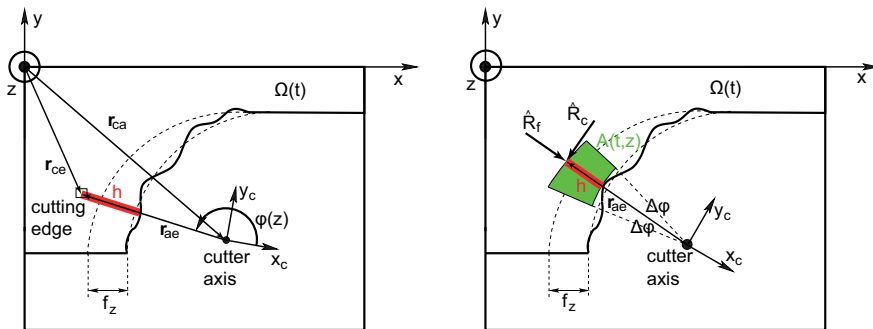
Figure 8: Uncut chip thickness (left) and definition of the volume force (right).
