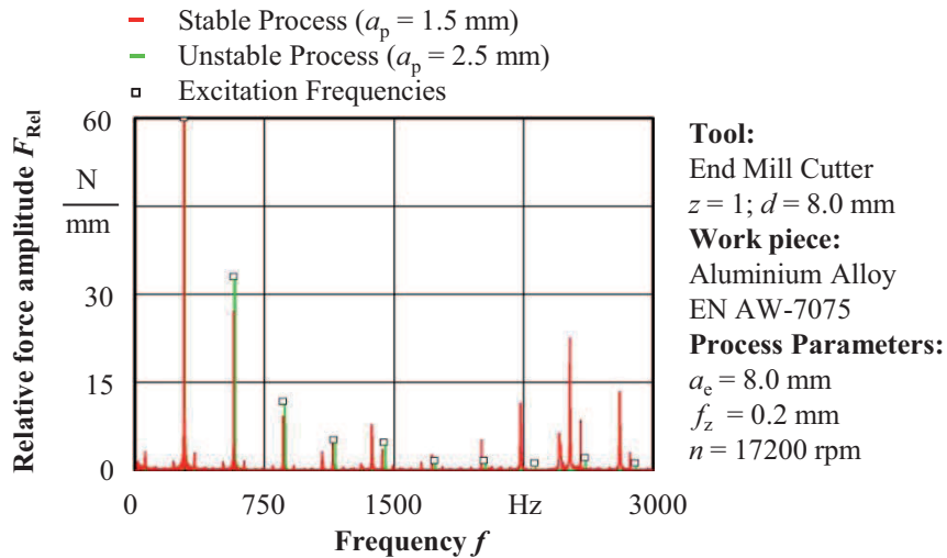
Figure 2: FFT of stable and unstable cutting processes.
