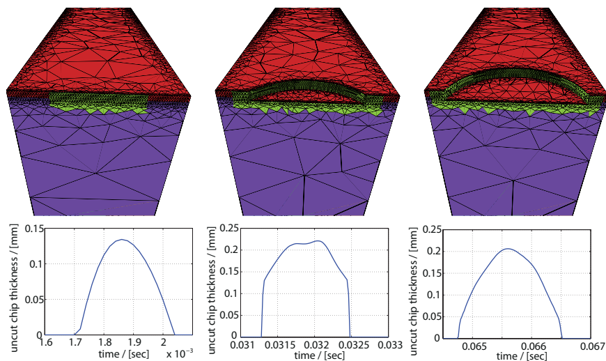
Figure 9: Example for the material removal simulation, i.e. the evolution of the work piece shape, and the corresponding uncut chip thickness in case of a stable cut.
