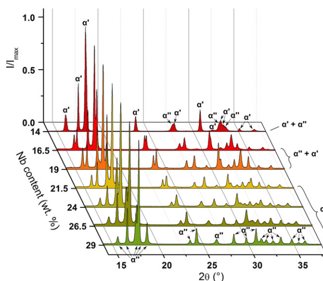
Figure 1. XRD-patterns of homogenized and water-quenched Ti–(14–29)Nb alloys.
