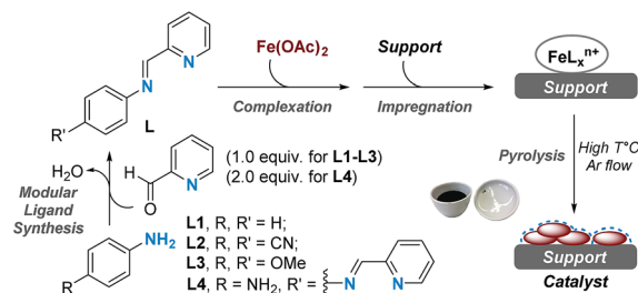
Scheme 1 General procedure for the synthesis of Fe-based materials.
