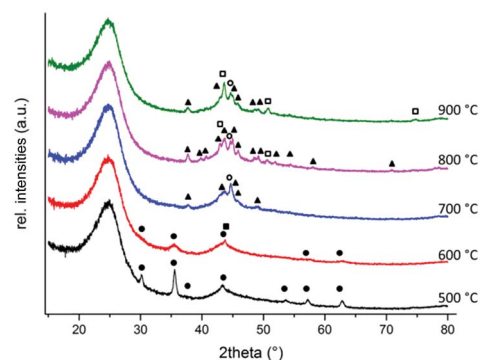
Fig. 3 Powder X-ray diffraction pattern of the Fe(1)/ L4 (1.5)@C-T catalyst at different pyrolysis temperatures ( T = 500 °C (black), T = 600 °C (red), T = 700 °C (blue), T = 800 °C (purple) and T = 900 °C (green)). Phases are shown as filled circles (Fe 3 O 4 , ICDD 01-084-2782), filled squares (Fe 3 C, ICDD 01-083-0878), triangles (Fe 3 N, ICDD 00-034-0001), empty circles (Fe, ICDD 00-006-0696), and empty squares (FeN x , ICDD 01-075-2127).
