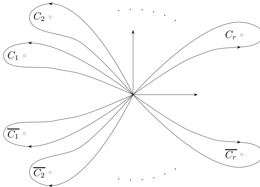
FIGURE 1. Monodromy representation of [A]
