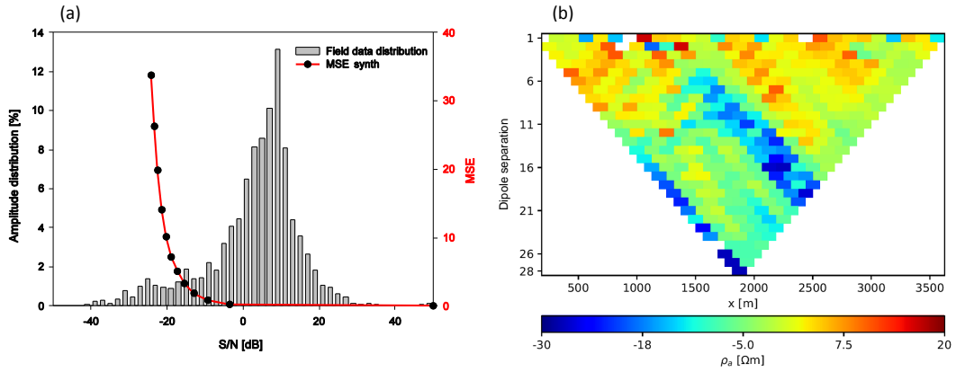
Figure 14. Signal-to-noise values of field data. (a) Histogram compared to MSE of synthetic data, (b) in a pseudo-section.
