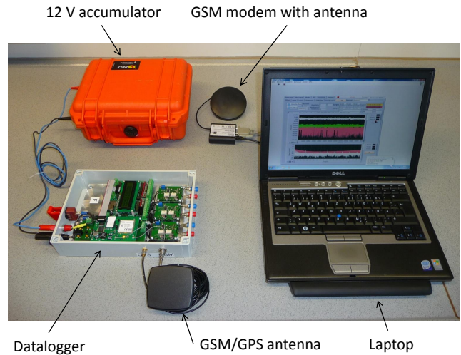
Figure 2. Datalogger system with datalogger, GSM/GPS antenna and 12 V accumulator. A laptop with GSM modem and antenna for remote control.
