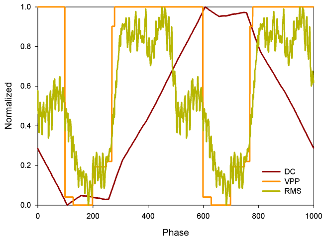
Figure 9. Evaluated functions of direct current (DC) value, peak-to-peak voltage V_{pp} and effective root mean square (rms) of the mask-convoluted signal.
