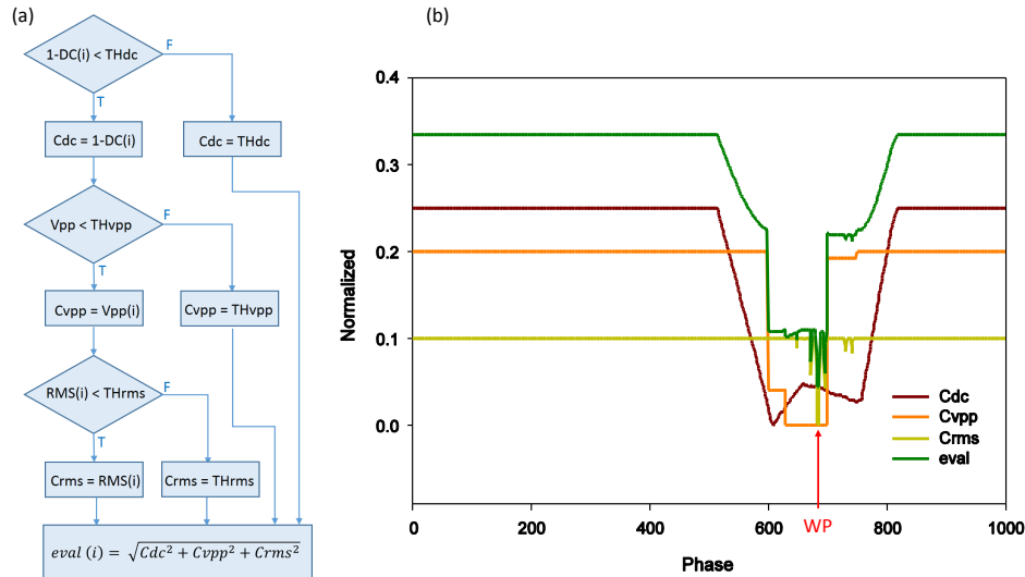
Figure 10. (a) Flow diagram calculation of the components C_{dc} , C_{vpp} and C_{rms} from the three functions. (b) Components and quadratic sum for calculating the working point (WP) from its minimum.
