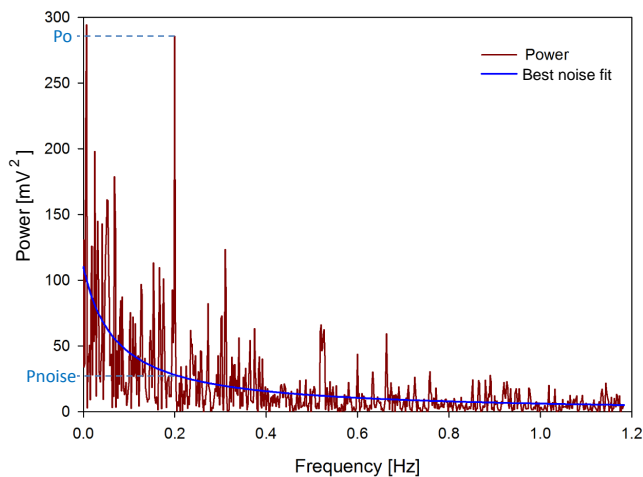
Figure 5. FFT-based fitting of a noise function ( P_{\text{noise}} ) and calculation of the signal strength ( P = P_o - P_{\text{noise}} ) at the first harmonic f = 0.2 Hz.
