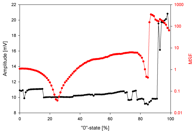
Figure 11. Detected amplitude and mean square error MSE of an artificial signal with 10 mV overshoot and 29 mVrms pink noise over length of 0 state, showing the plateau between 16 and 35 %. Up to 16 % 0 state is the effect of the overshoot; above 70 % is the reduced noise rejection.
