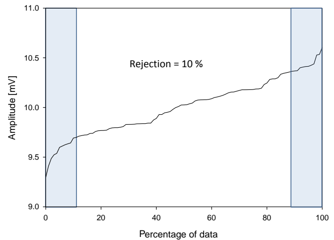
Figure 6. Sorted amplitude distribution for the alpha-trimmed-mean stacking.
