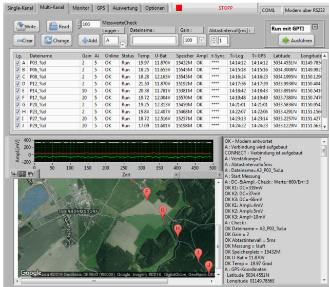
Figure 3. Software GUI in multi-channel mode.
