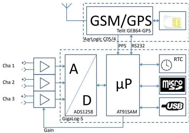
Figure 1. Block diagram of datalogger consisting of a GigaLog-S data acquisition module, a combined GSM/GPS modem and three preamplifiers.
