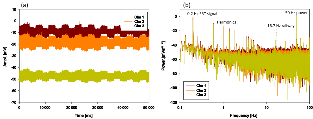
Figure 4. Exemplary voltage time series (a) from a square-wave current injection and frequency spectrum (b) as visible in the GUI monitoring software.
