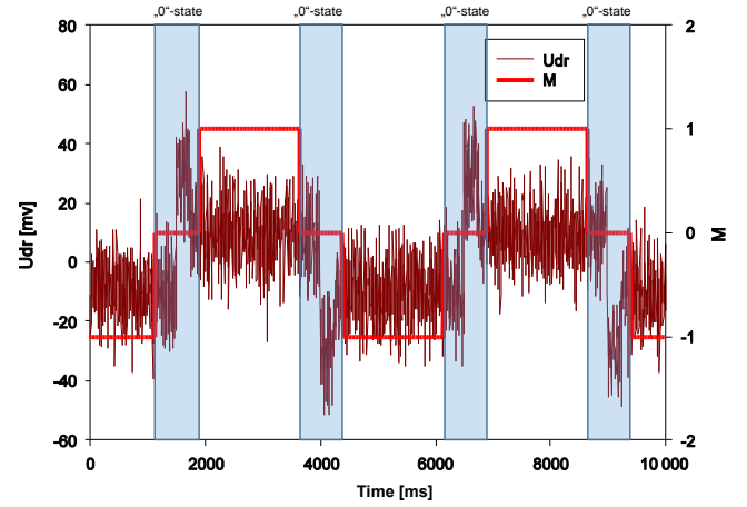
Figure 8. Drift-corrected signal U_{dr}(t) and mask signal M(t) in correct phase.
