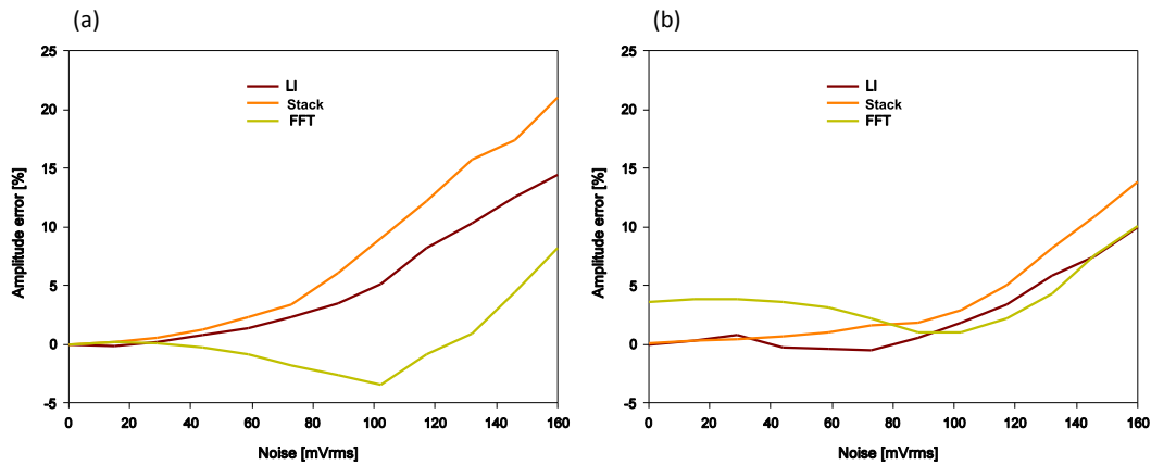
Figure 13. (a) Comparison of LI, stack and FFT over pink noise without overshoot. (b) Comparison of LI, stack and FFT over pink noise with overshoot.
