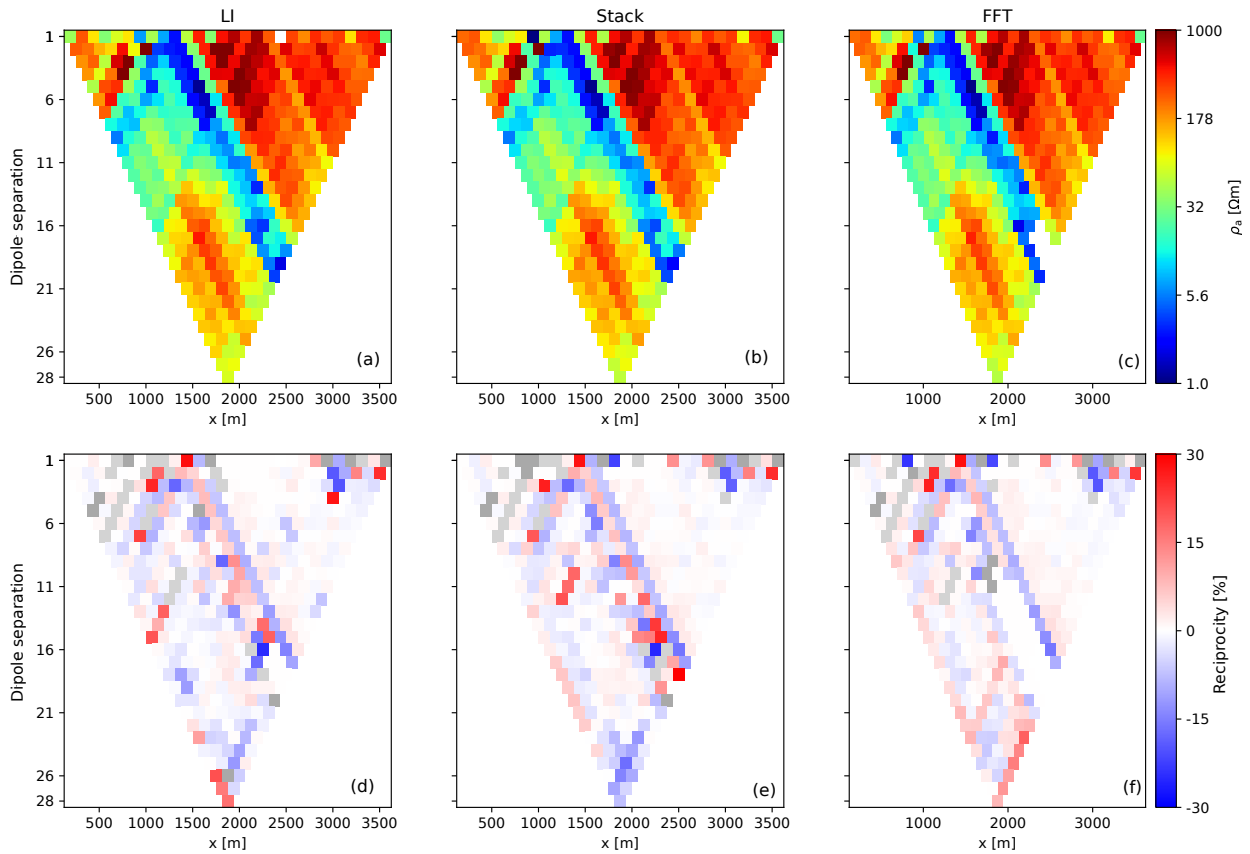
Figure 15. Calculated apparent resistivity (a, b, c) and normal reciprocity (d, e, f) for the three analysis approaches, lock-in (a, d), stacking (b, e) and FFT (c, f).
