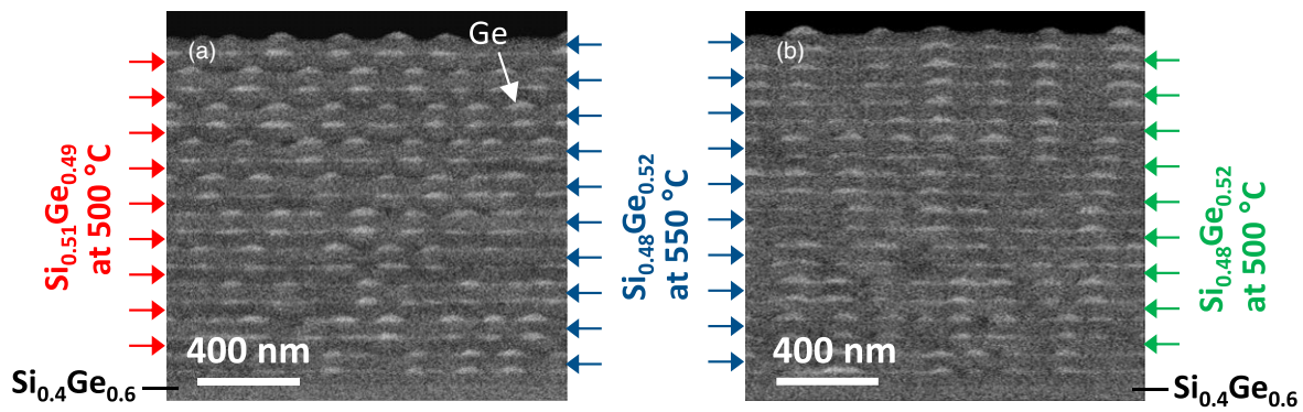
Fig. 3. (Color online) Cross section SEM images of 20-cycle SL of 52 nm SiGe/12.5 nm Ge. Si 0.48 Ge 0.52 grown at 550 °C and (a) Si 0.51 Ge 0.49 or (b) Si 0.48 Ge 0.52 grown at 500 °C alternately used as spacers.
