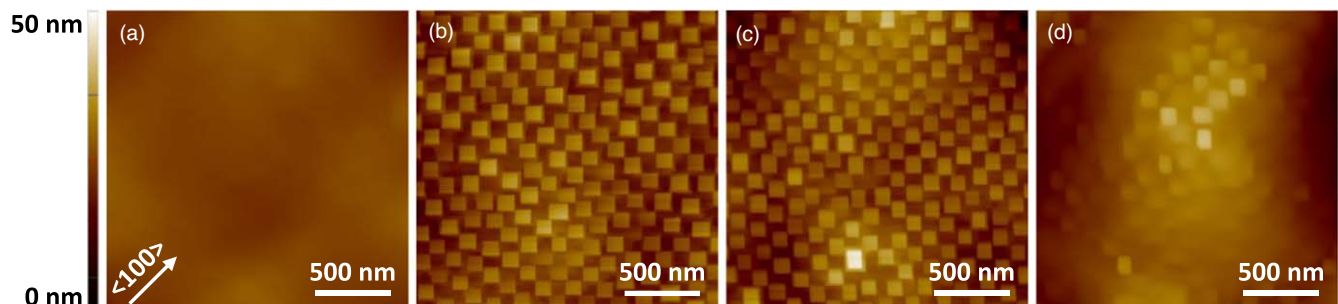
Fig. 1. (Color online) AFM images of 52 nm (a) \text{Si}_{0.51}\text{Ge}_{0.49} grown at 550 °C, (b) \text{Si}_{0.55}\text{Ge}_{0.45} , (c) \text{Si}_{0.51}\text{Ge}_{0.49} and (d) \text{Si}_{0.48}\text{Ge}_{0.52} grown at 500 °C on laterally ordered Ge nanodot templates.
