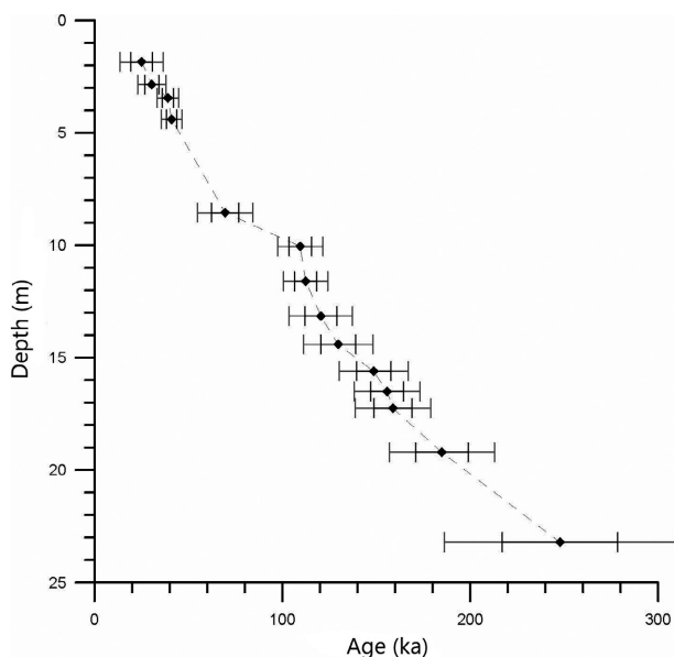
Fig. 9. Age modelling results and pIRIR 200, 290 ages from Nosak. The results were obtained using the ADmin age-depth modelling method specifically developed for treating luminescence data (Zeeden et al. 2018). The original data and uncertainty are plotted as diamonds with error bars: 1-sigma uncertainty as a black line and 2-sigma uncertainty as a grey line. Mean age and uncertainty were linearly interpolated between the age-depth points used in the modelling.
