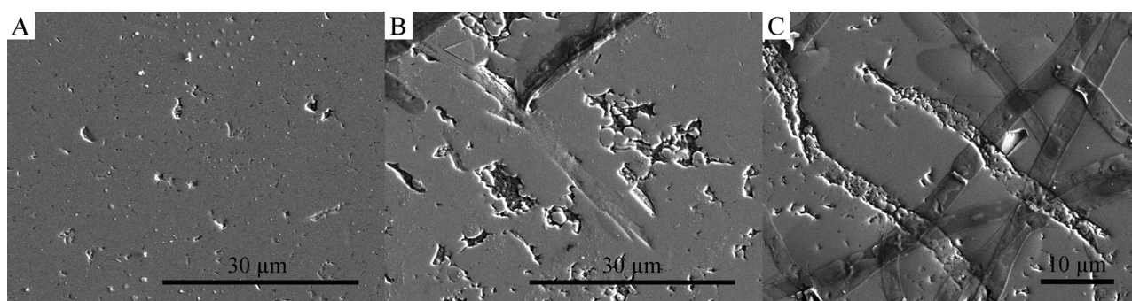
Fig. 5. Polished black slate pieces with a non-inoculated control showing naturally occurring depressions of the rock topography (A) and overgrown black slate samples showing etch pits of hyphae produced by S. commune EVC (B) and S. commune lcc2-OE (C). Typical images are shown.
