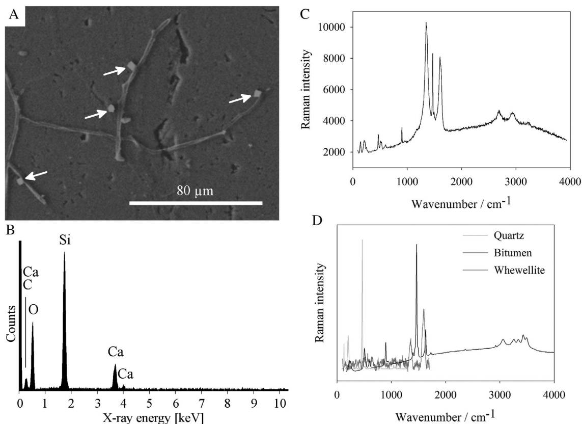
Fig. 4. Identification of biominerals. Biominerals produced on the hyphae of S. commune lcc2-OE (A, arrows) and analysis of the biominerals through EDX analysis (B). Raman spectrum of a biomineral (C) and reference spectra for bitumen, quartz and whewellite (D). Typical data are shown from several determinations.
