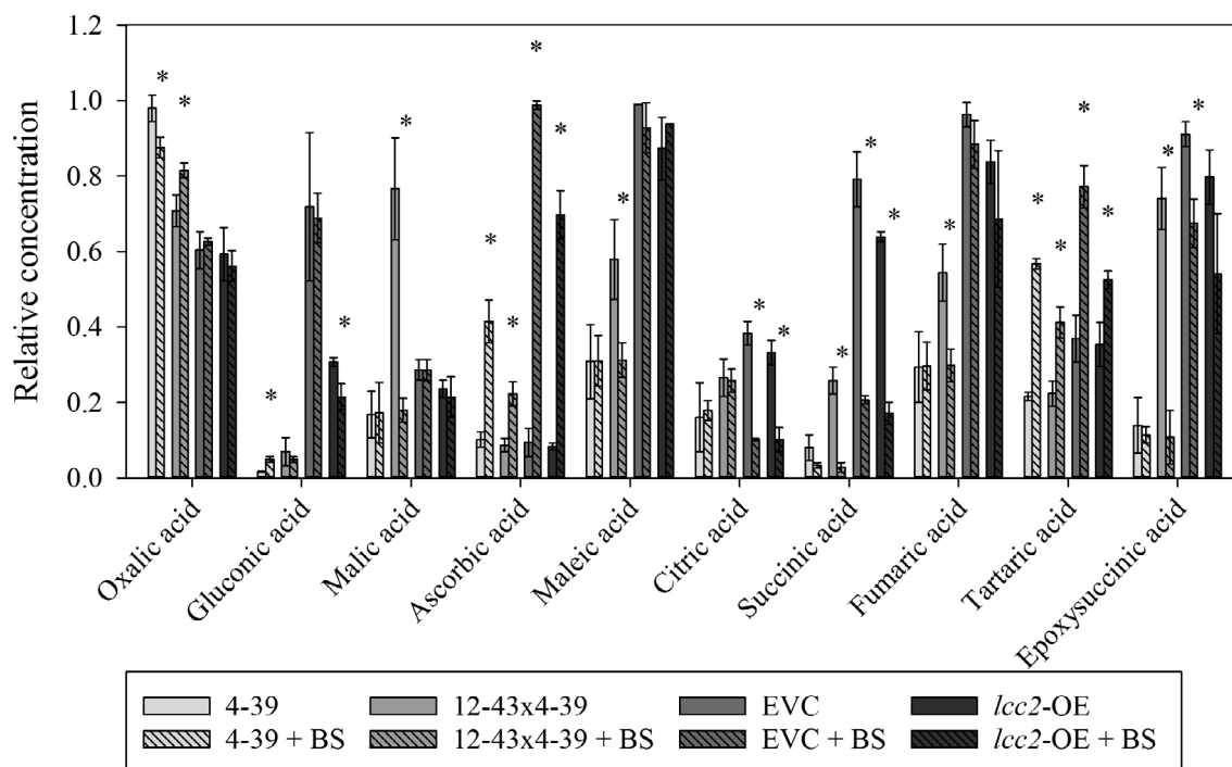
Fig. 6. Organic acids production and black slate-induced changes (BS) by different strains, the unmated monokaryon S. commune 4–39, a mated dikaryon S. commune dikaryon 12-43 × 4-39, empty vector control transformant S. commune EVC and laccase overexpressing S. commune lcc2-OE. Error bars indicate standard deviation; * p < 0.03 , paired, two-tailed t -test.
