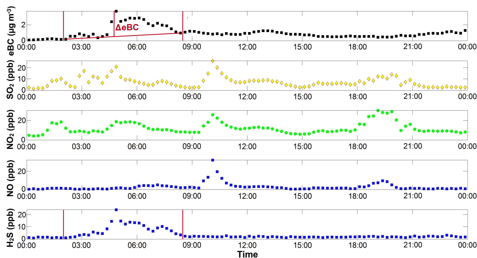
Figure 3. Example to illustrate how species were correlated with eBC in order to separate sources from one another. The excess eBC ( \Delta eBC ), defined as the eBC concentration above the baseline for this example, is also indicated in the top panel.
